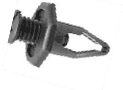
Grapa Tipo Tornillo Chrysler / Honda L: 24mm Ø: 10mm Head: 20mm
